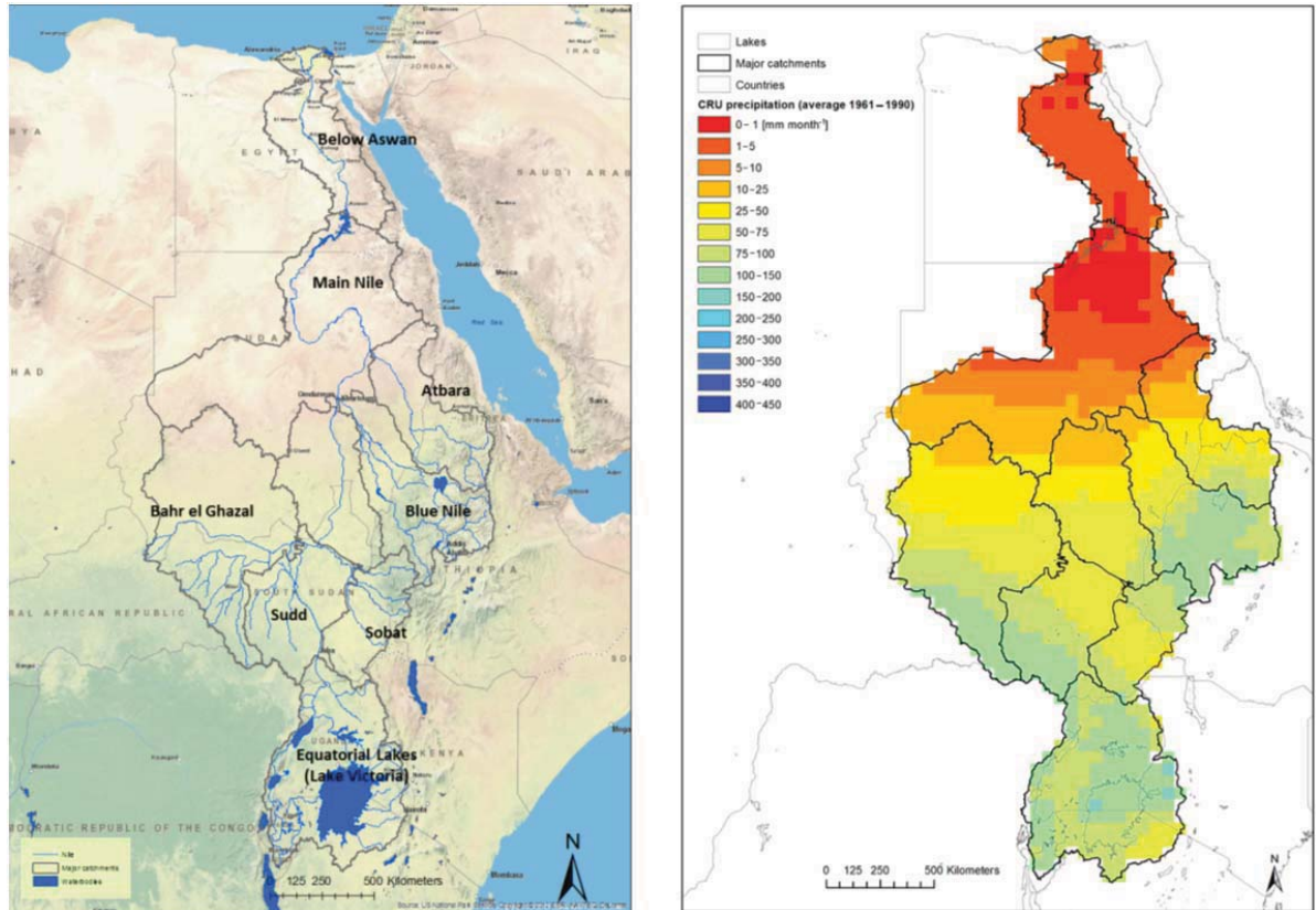
Figure 2: An overview of the Nile Basin (left) and distribution of annual average rainfall in mm/month for the period 1961–1990 (right), from CRU (Harris et al., 2014).
