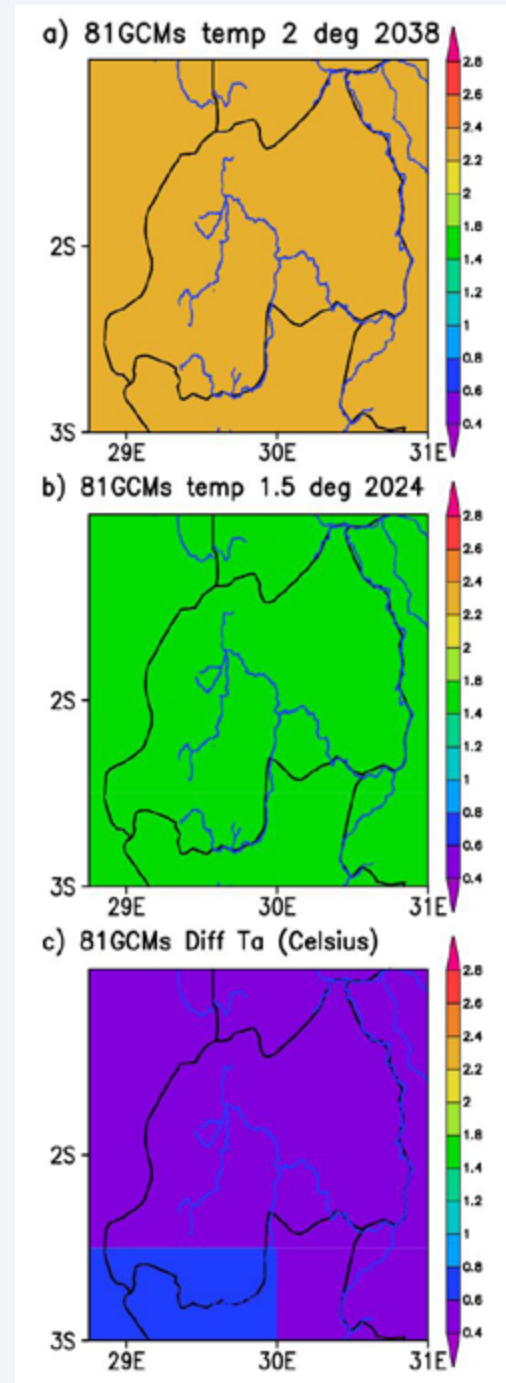
Figure 6: Projected spatial annual temperature change for Rwanda, at the time of global warming of 2°C, 1.5 °C, and the difference. Data are average from 81 CMIP5 climate model simulations under the RCP8.5 forcing scenario.
