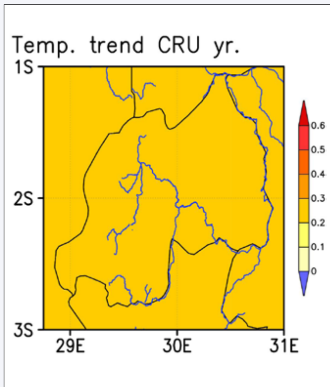
Figure 4: The monotonic slope in temperature (deg C) between 1963 and 2012 at each grid cell, according to a linear trend per decade for Jan to Dec. Hatching indicates areas where the trend is not statistically significant at the 95% level. Data taken from the CRU TS3.22 datasets.
