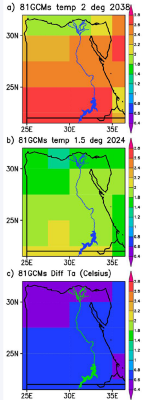
Figure 6: Projected spatial annual temperature change for Egypt, at the time of global warming of 2°C, 1.5 °C, and the difference. Data are average from 81 CMIP5 climate model simulations under the RCP8.5 forcing scenario.
