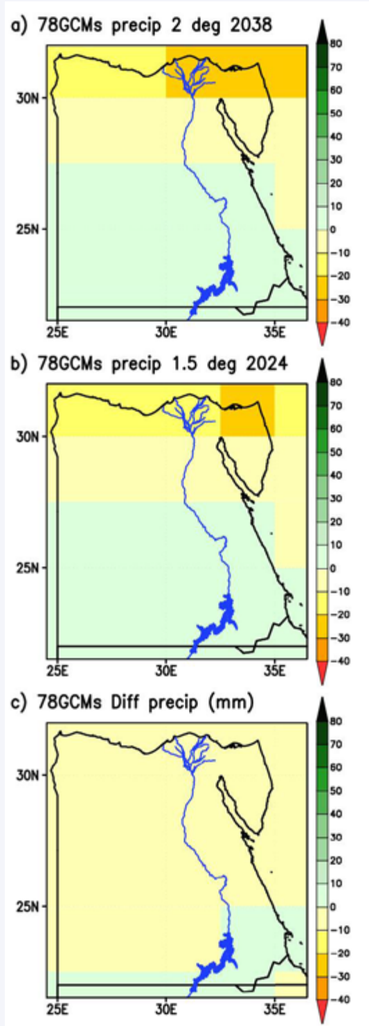
Figure 5: Projected spatial annual rainfall change for Egypt, at the time of global warming of 2°C, 1.5 °C, and the difference. Data are average from 78 CMIP5 climate model simulations under the RCP8.5 forcing scenario.
