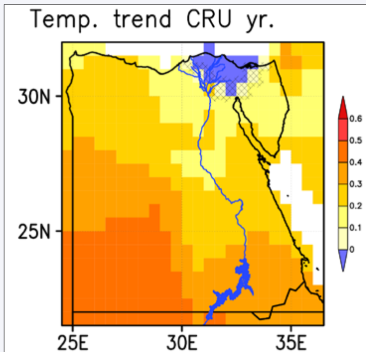
Figure 4: The monotonic slope in temperature (deg C) between 1963 and 2012 at each grid cell, according to a linear trend per decade for Jan to Dec. Hatching indicates areas where the trend is not statistically significant at the 95% level. Data taken from the CRU TS3.22 datasets.
