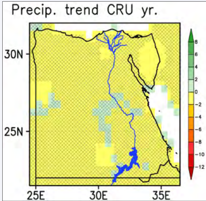
Figure 3: The monotonic slope in precipitation (mm) between 1963 and 2012 at each grid cell, according to a linear trend per decade for Jan. to Dec. Hatching indicates areas where the trend is not statistically significant at the 95% level. Data taken from the CRU TS3.22 datasets.
